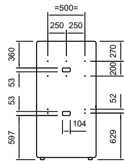
1600 High Connector Wall fixings & cut out positions.
